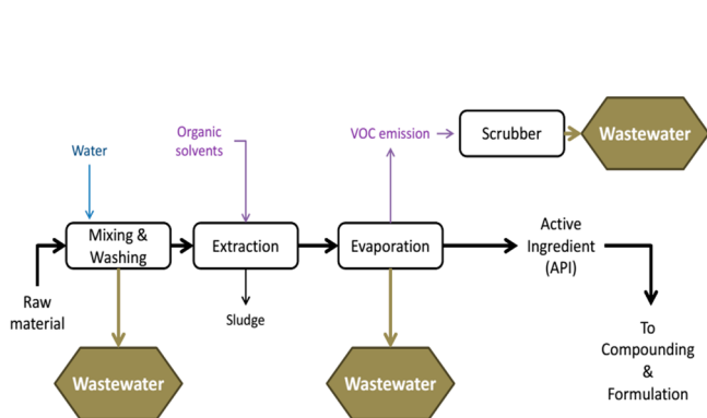
Figure 5. Process flow sheet diagram for natural/biological extraction process. Adapted from ref 29. Copyright 1998 U.S. EPA.
